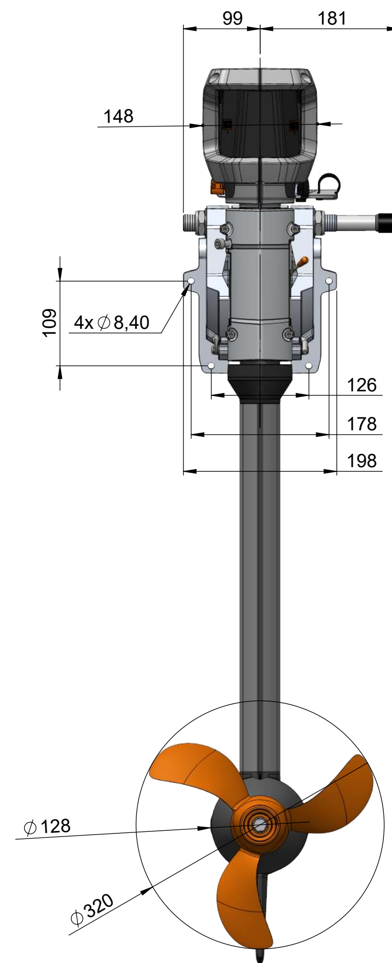
Cruise 6.0 Standard Propeller B 12,5x17 HSP [1987-00]
